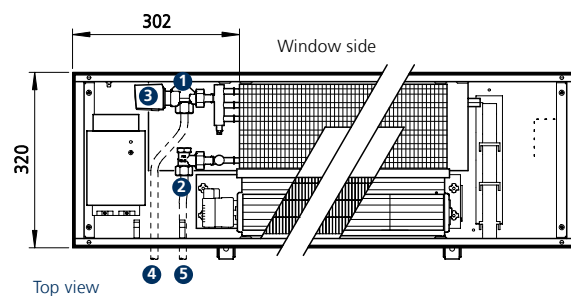
Katherm HK 320/130, 2-pipe, trench height 130 mm
