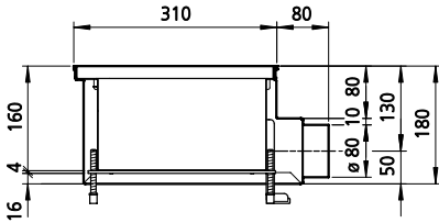
Side view of HK 290 with primary air modules
