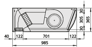
Cross-section
