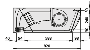
Cross-section
