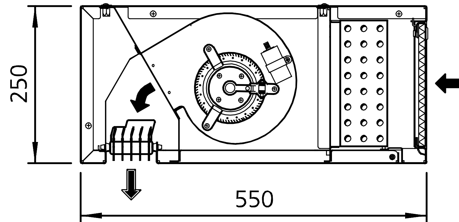
Cross section
