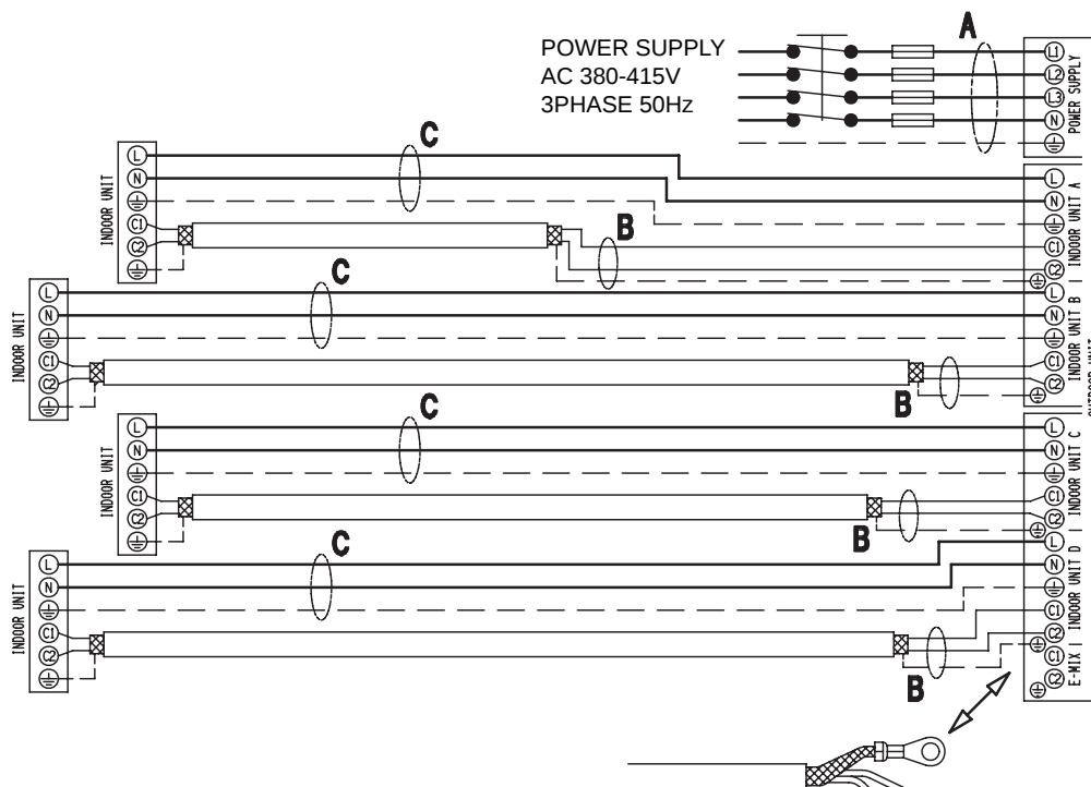
4 INDOOR UNITS 3 PHASE
