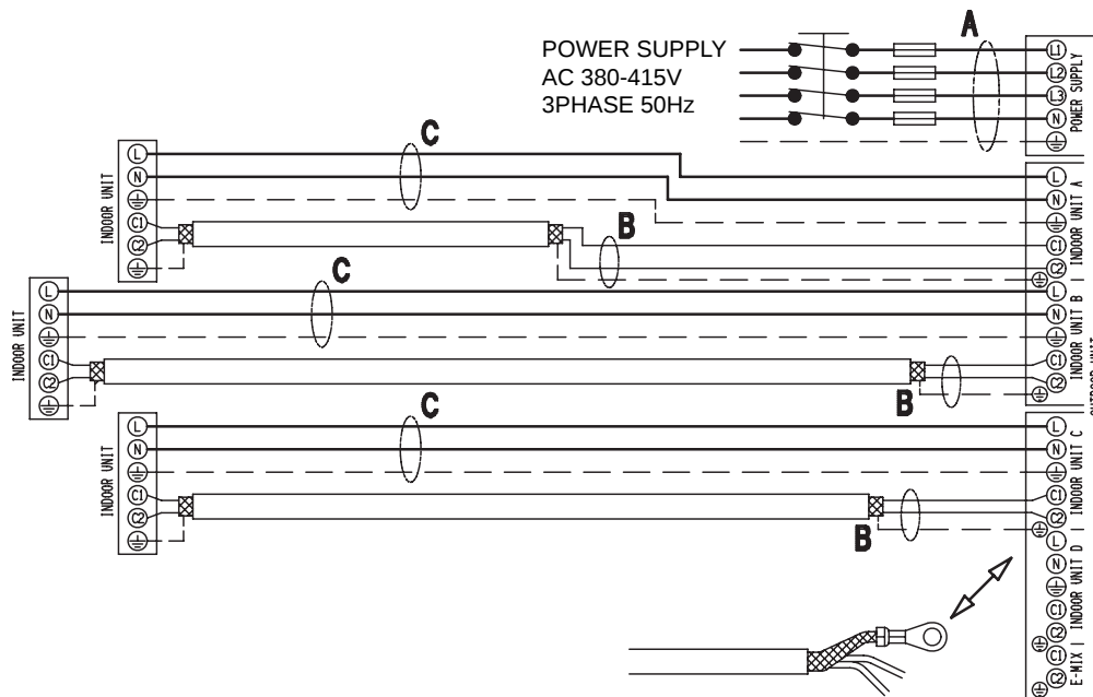
3 INDOOR UNITS 3 PHASE
