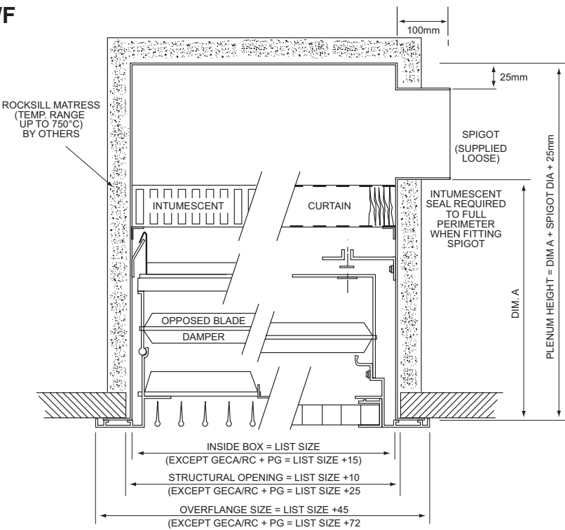
Grille c/w Damper
