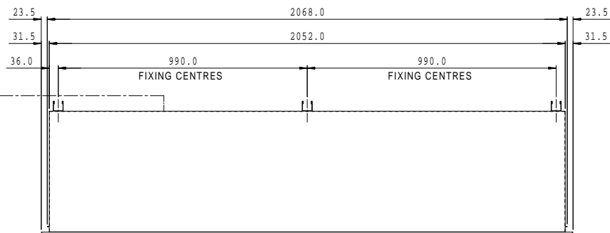
FRONT VIEW
