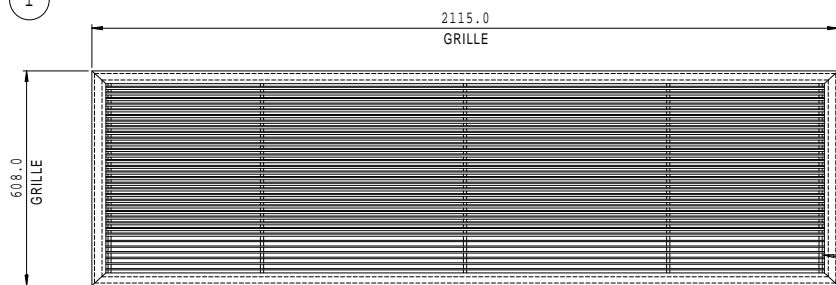
UNDERSIDE VIEW
